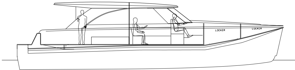
Targa Profile
