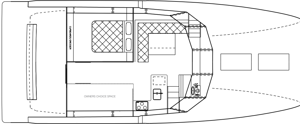
Bridgedeck Plan
