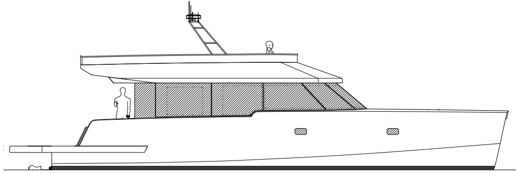
Flybridge Profile
