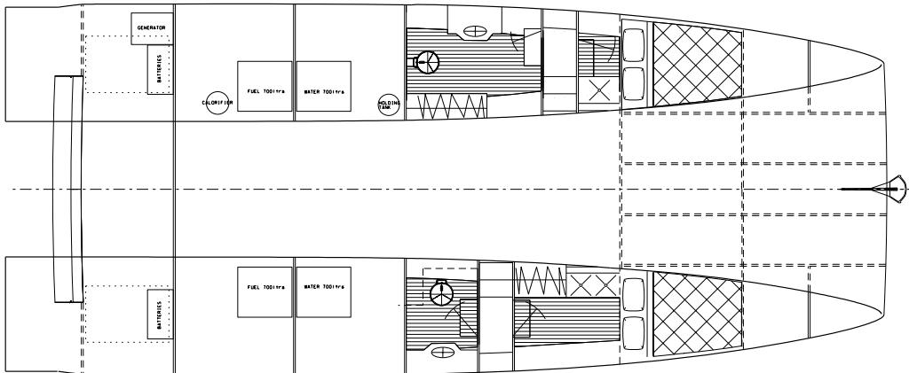
Hulls Plan
